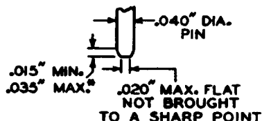
Pin Contour
