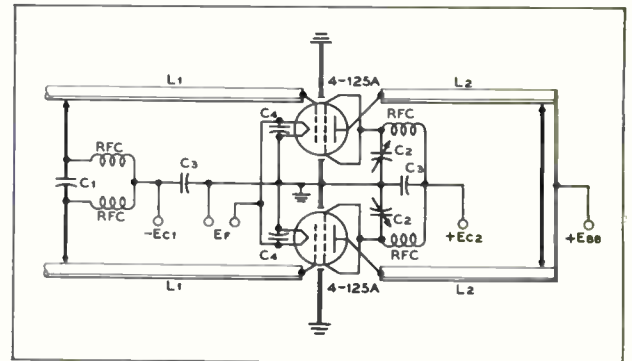
Typical circuit arrangement useful for frequencies above 175 Mc. C 1 —See above. C 2 —Neutralizing capacitor. C 3 —.001 μfd. C 4 —100 μfd. L 1 —3/8" dia. copper spaced 1" center-to-center, 6" long. L 2 —7/8" dia. brass, silver plated, spaced 1 1/2" center-to-center, 14" long.
