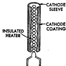
Fig. 2—Indirectly heated cathode or heater-cathode.
