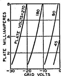
Fig. 13—Family of transfer-characteristic curves.
