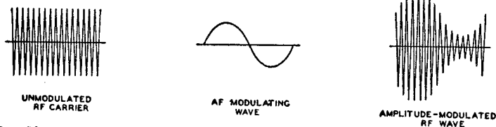
Fig. 50—Waveforms showing effect of amplitude modulation on an rf wave.
