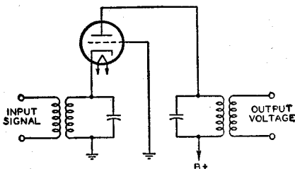
Fig. 27—Cathode-drive circuit.
