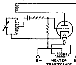
Fig. 75—Tuned-grid triode oscillator circuit using heater-cathode-type tube.
