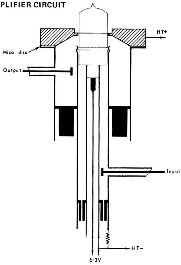
Fig. 5 AMPLIFIER CIRCUIT
