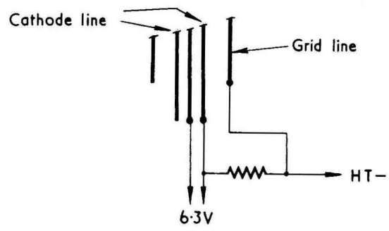
Fig. 6 The Circuits of Figs. 4 and 5 Modified for Cathode Bias
