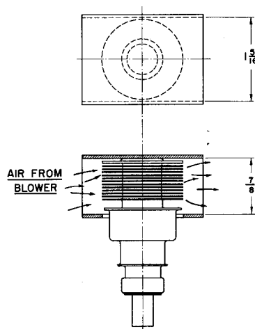
RECOMMENDED COWLING FOR FORCED-AIR COOLING OF ANODE
