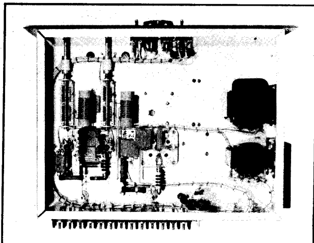
FIG. 4—Bottom view of the r-f section chassis. All r-f circuits preceeding the 4-250A plate circuit are placed under the chassis, to prevent unwanted feedback around the power amplifier stage. Holes in the 4-250A socket allow adequate circulation of air through the tube base, with the aid of the exhaust fan above the chassis.
