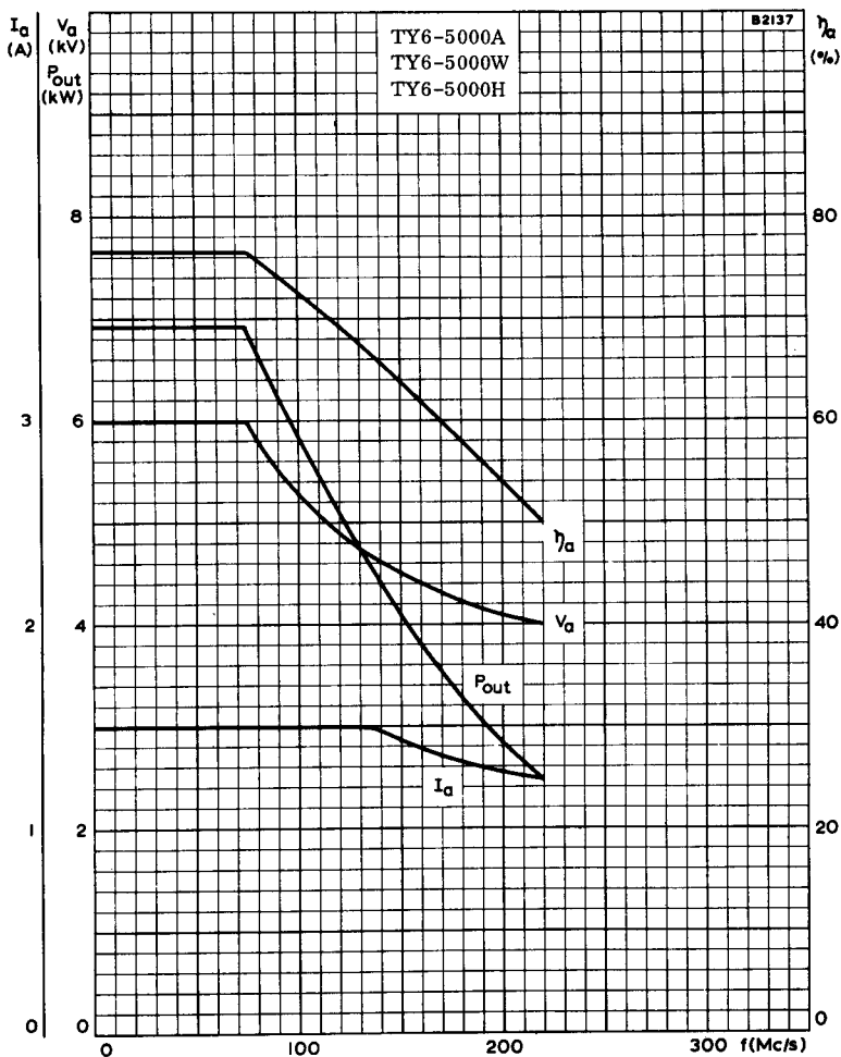
FREQUENCY CHARACTERISTICS
