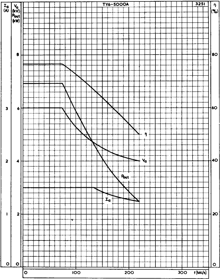
FREQUENCY CHARACTERISTICS
