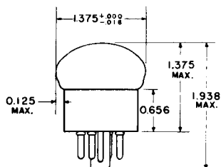
TUBE DIMENSIONS
