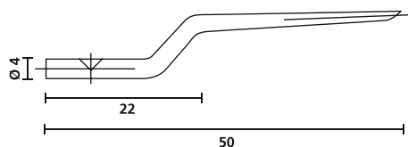
Replacement prong NA1K/3
