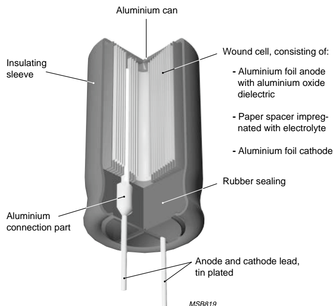
Fig.4 Radial Aluminium.
