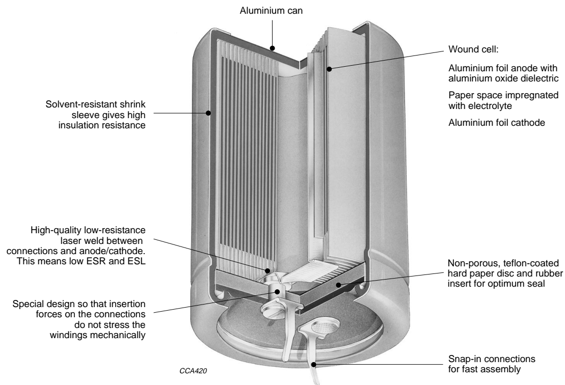
Fig.6 Large Aluminium, snap-in.
