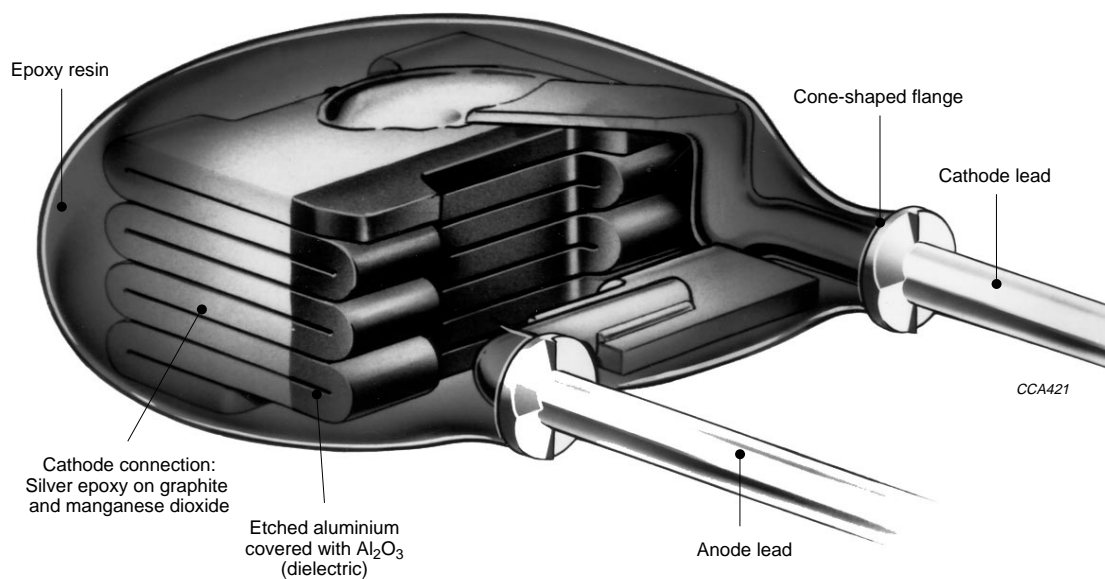
Fig.7 Solid Aluminium (SAL), radial.
