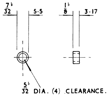
1/2" DIA. PULLEY SPACER.
