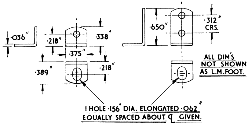
M.O.S. FOOT. PART No. 4378
