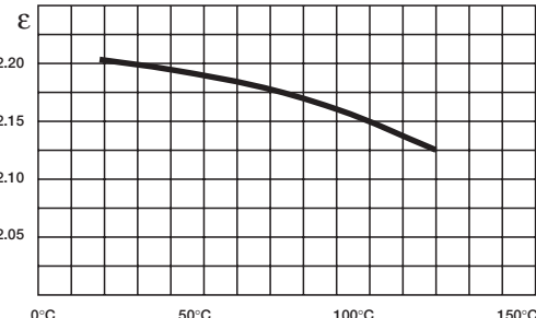
Costante dielettrica Dielectric constant
