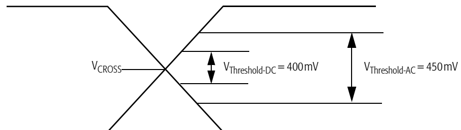
Figure 11. SYSCLK and SYSCLK# Differential Clock Signals
