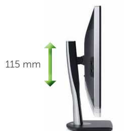
Height adjustment
