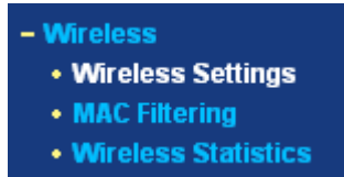
Figure 5-14 Wireless menu
