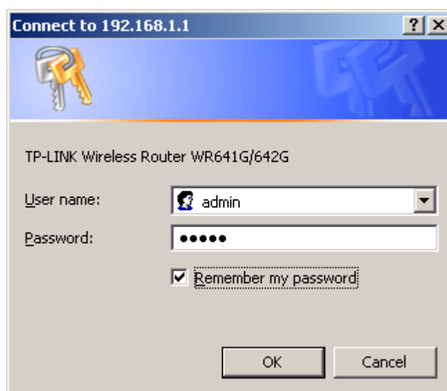
Figure 4-4 Login Windows
