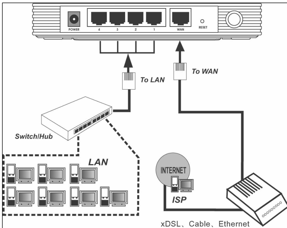
Figure 3-1 Hardware Installation of the TL-WR642G 108Mbps Wireless Router
