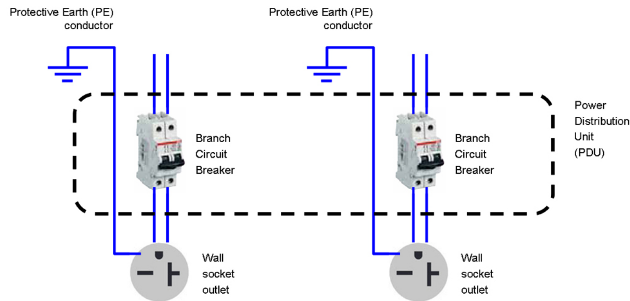
Figure 2-1 Electrical configuration diagram
