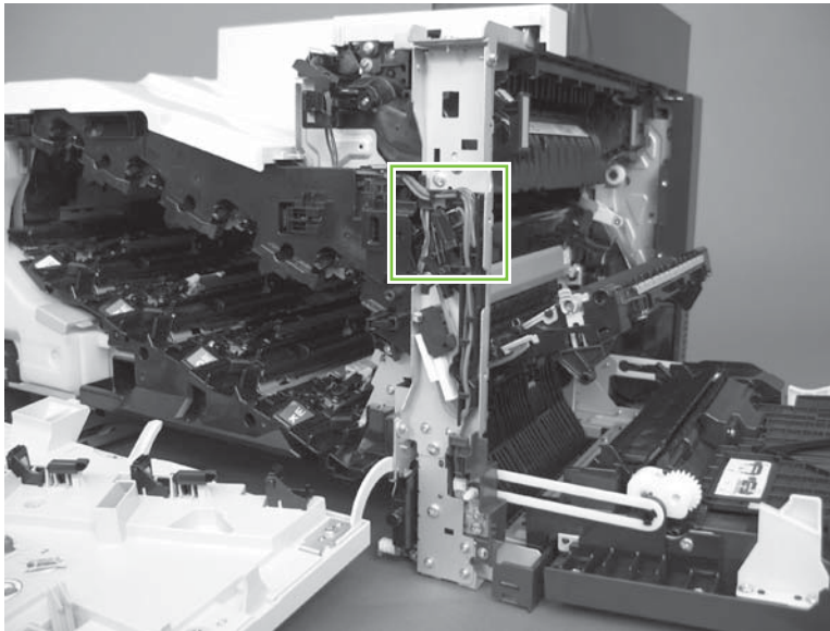
Figure 7-17 Test the right- and front-door interlock switches (4 of 4)
