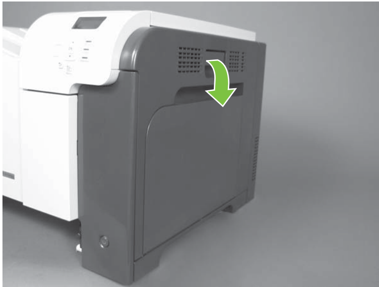
Figure 6-77 Remove the right-rear cover (1 of 3)
