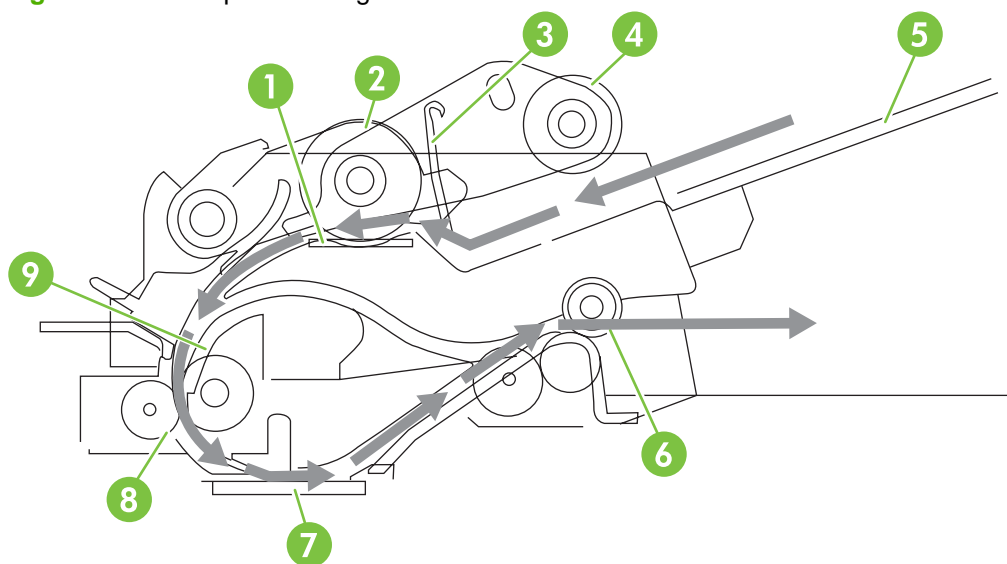
Figure 5-51 ADF path for single-sided documents
