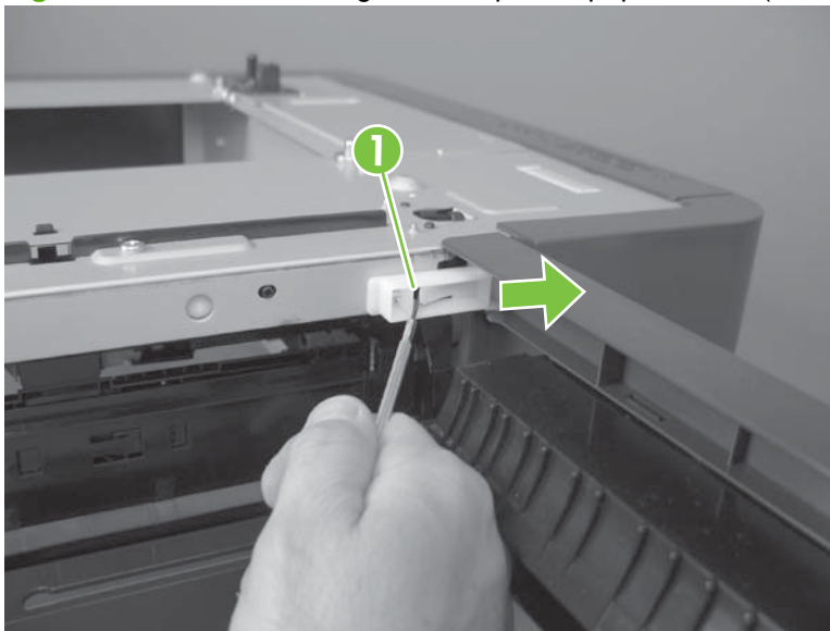
Figure 6-62 Remove the right door; optional paper feeder (2 of 3)
