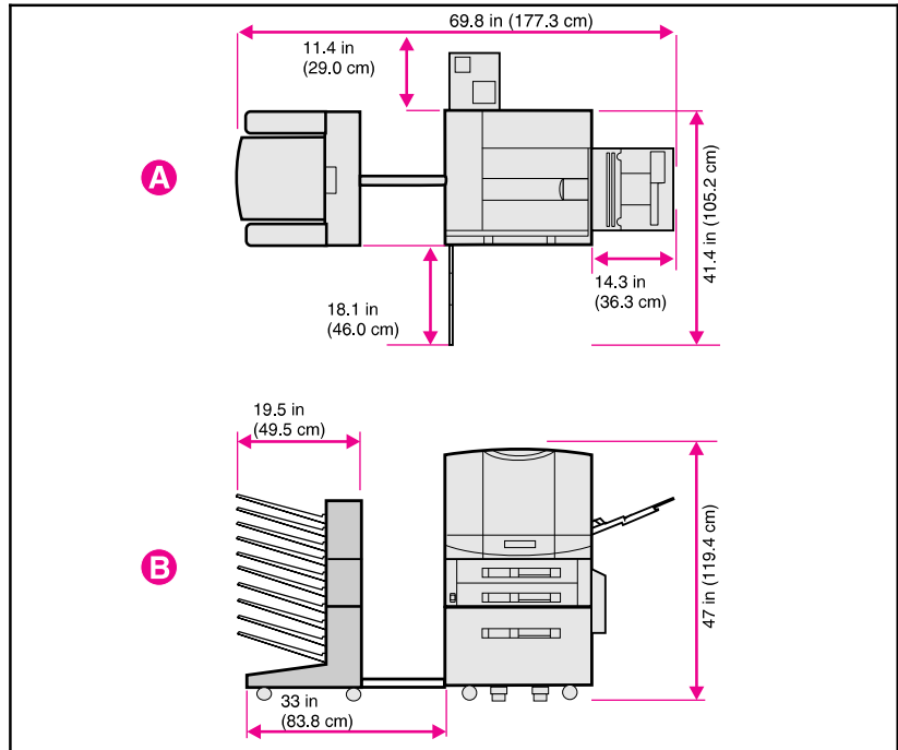
A Top View (with optional multi-bin mailbox and tray 4) B Front View (with optional multi-bin mailbox and tray 4)
