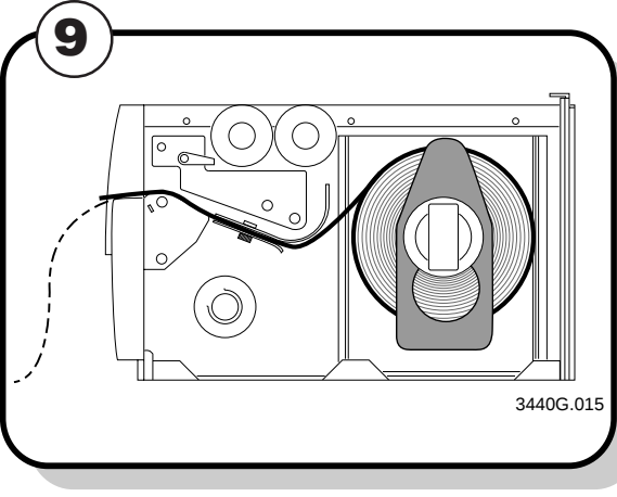
Unroll several inches of media and route it through the printer mechanism.
