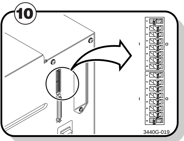
Enable thermal transfer printing by setting DIP switch 8 on the bottom bank of switches to the on (1) position. Turn the printer power off and then on to activate the new setting.
