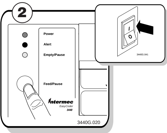
Press and hold the Feed/Pause button. Turn the On/Off switch to the on (I) position.
