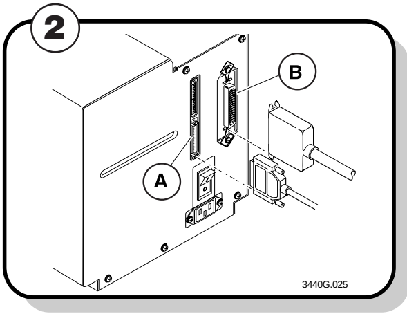
Plug the 25-pin connector into the serial (A) or parallel (B) communications port on the rear of the printer.
