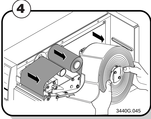
Remove the media and ribbon if necessary.
