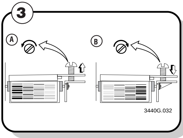
To compensate for uneven print quality, turn the bias adjust screw as shown.
