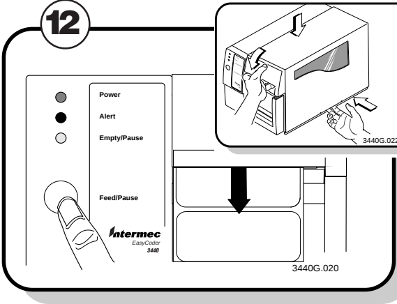
Press the Feed/Pause button to advance one label through the printer. Replace the media cover.
