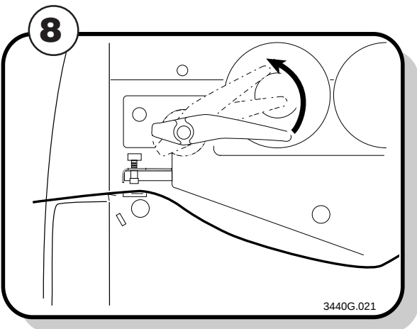
Lower the printhead by turning the head lift lever counterclockwise until it locks.
