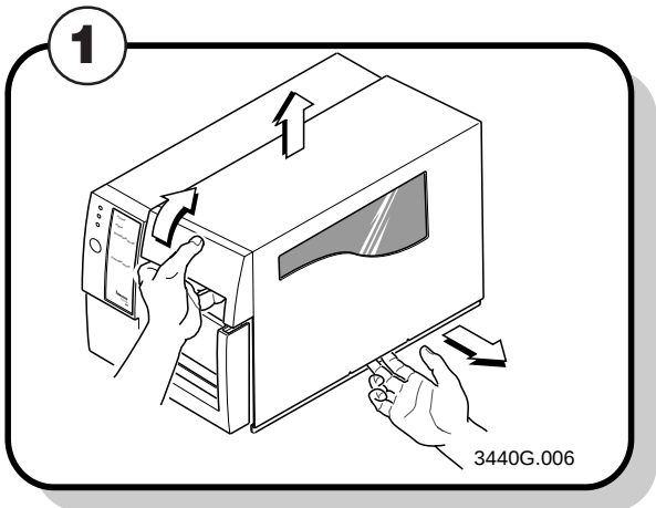
Remove the media cover.
