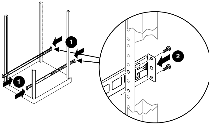
Figure 20 Installing the rack rails in rear of rack
