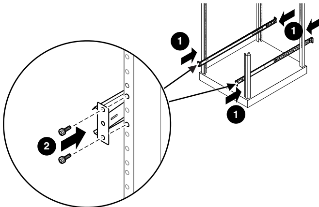
Figure 19 Installing the rack rails in front of rack
