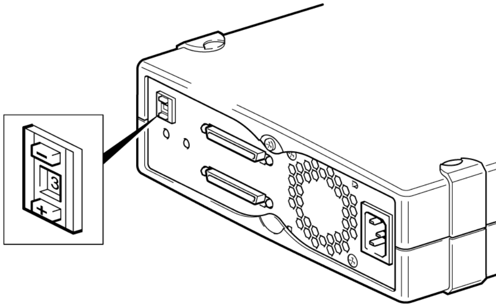
Figure 12 Setting the SCSI ID
