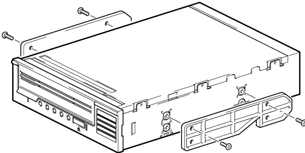
Figure 1 Attaching mounting rails
