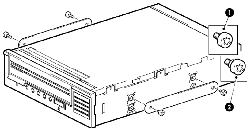
Figure 2 Attaching locating screws on a full-height drive
