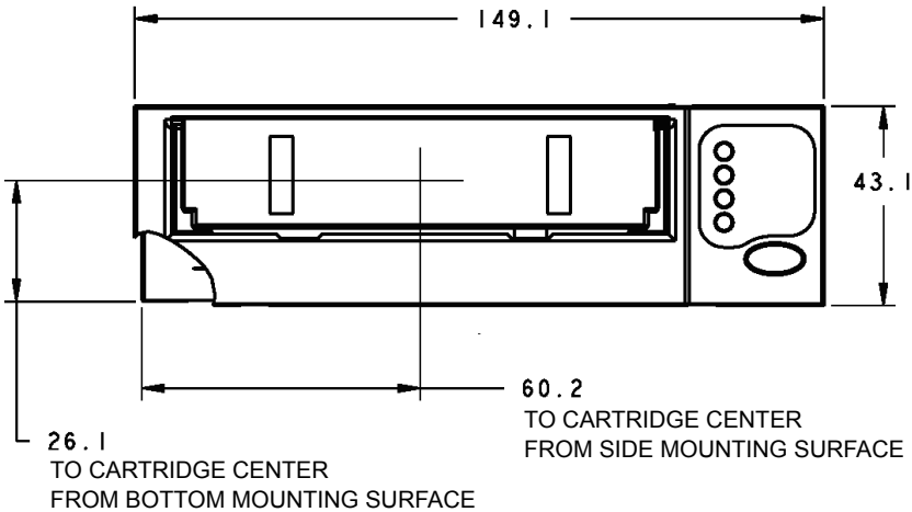
Figure 15 LTO-3 Half-Height Tape Drive Dimensions
