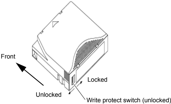
Figure 13 Ultrium Tape Cartridge Write-Protect Switch
