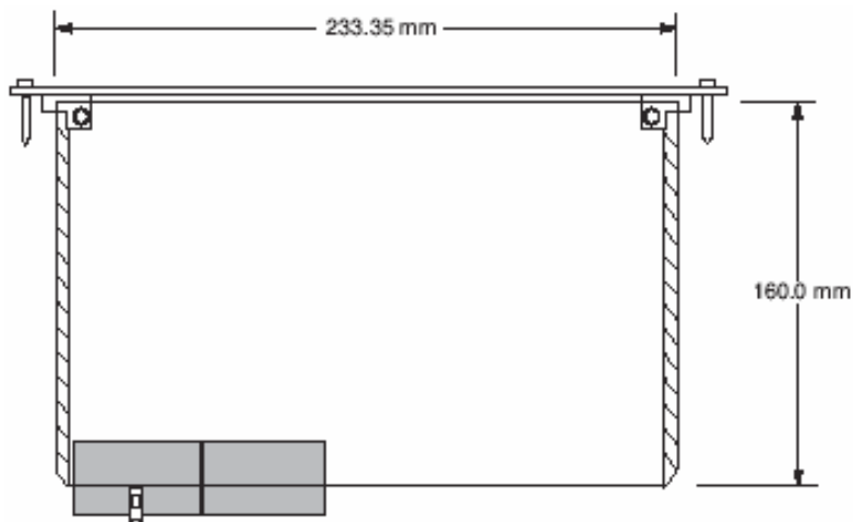
Figure 6. Board Dimensions
