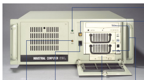
HDD LED Power switch One 3.5" drive bay Three 5.25" drive bays
