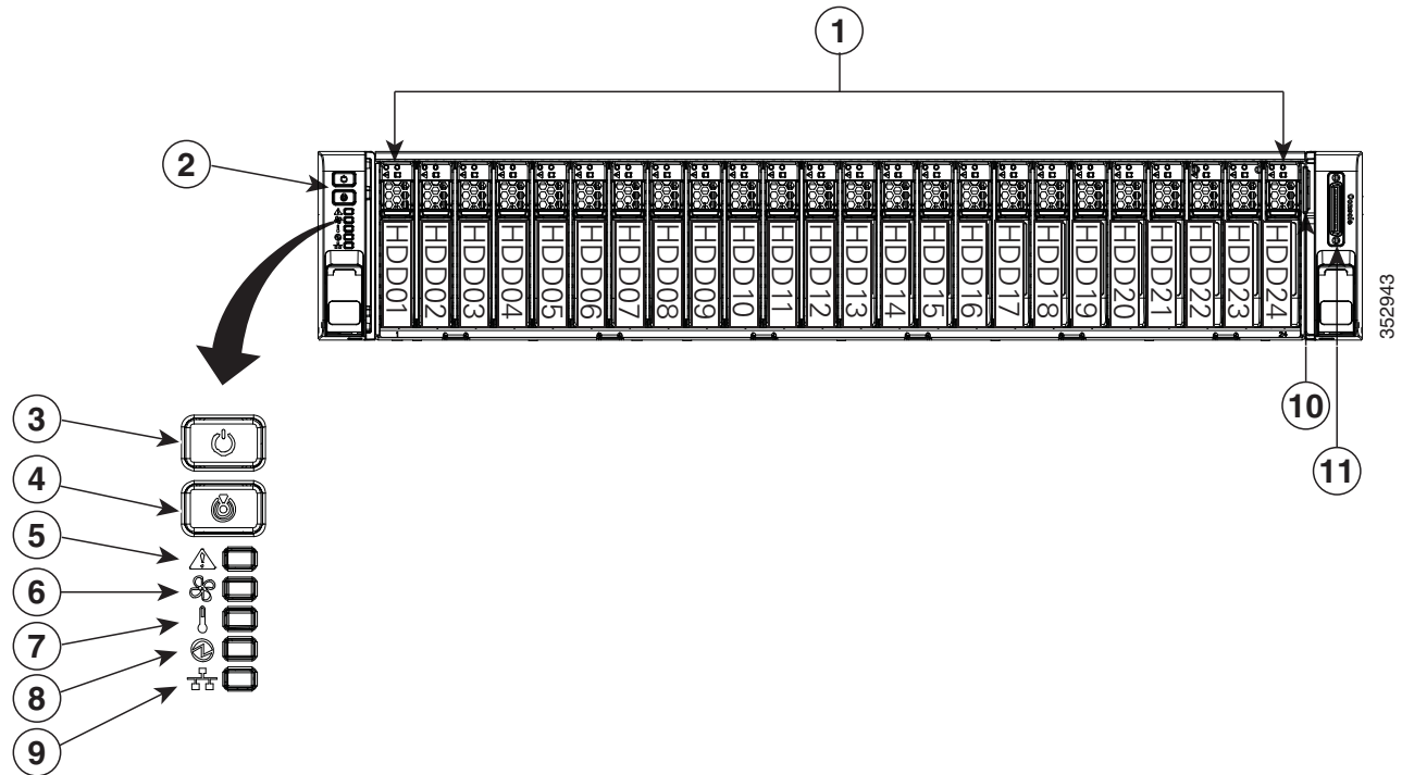
Figure 2 Chassis Front View (24-drive version)
