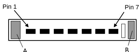
Figure 5-1. 7-Pin SATA Connector (P60-P64 on system board).
