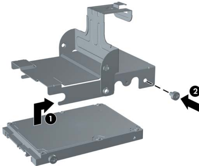
Figure 2-21 Installing the Hard Drive in the Carrier
