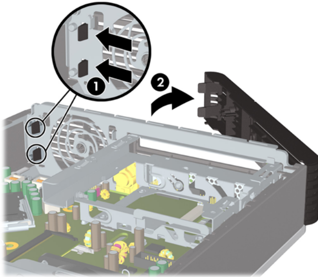
Figure 2-5 Removing the Front Bezel
