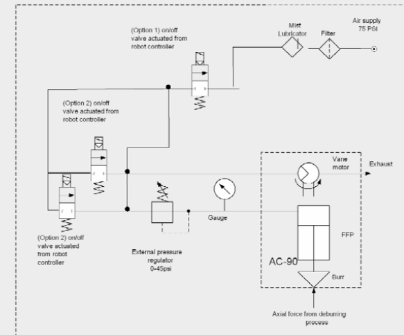
Pneumatic Diagram
