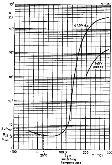
Resistance/temperature characteristic
