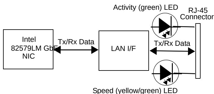
Figure 5-10. Network Interface Controller Block Diagram
