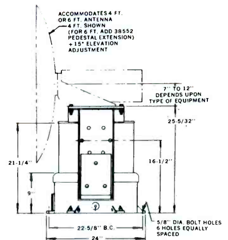
Type 38502 Shown With Typical "L" Bracket and TV Relay Unit.
