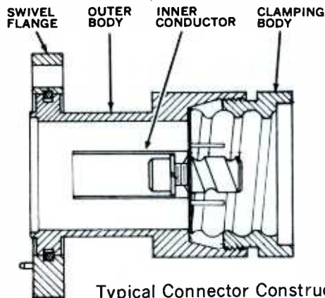
Typical Connector Construction
