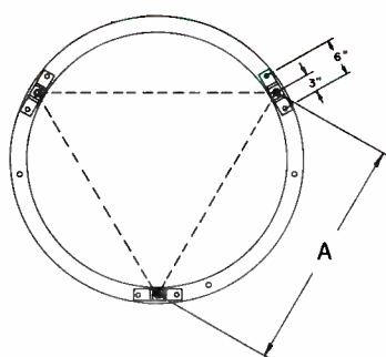
Type M10 Horizontal Mount for use with 4, 6, 8 and 10 foot antennas consists of 3 adjustment bolt assemblies and
