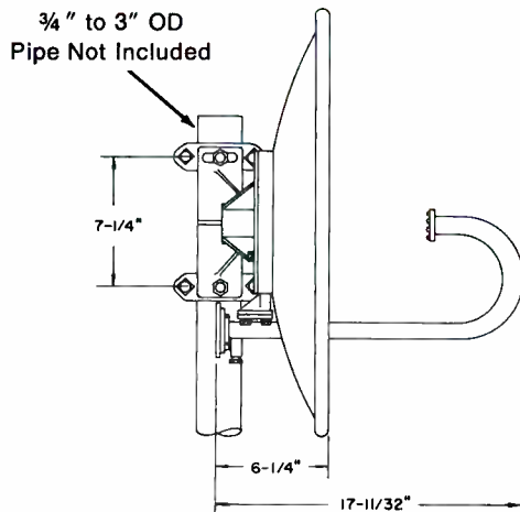
The 2 foot antennas include an integral clamp mount for attachment to a 3/4" to 3" OD pipe.
