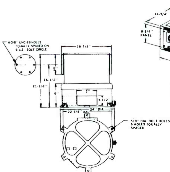
Remote Control Unit For Type 38500
