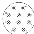
18-1 B,C,F,G=A; Bal.=Inst. 10 x #16
