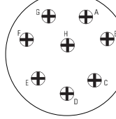
24-6 A,G,H=D; Bal.=A 8 x #12
