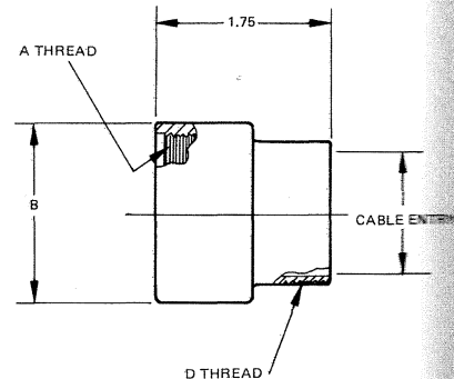
TYPE R, STRAIGHT
