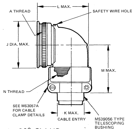
TYPE A 90° CLAMP
