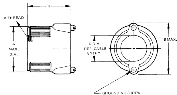
TYPE N NO CLAMP
