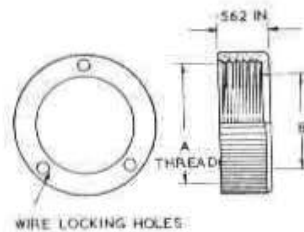
Fig. 32. Coupling unit
