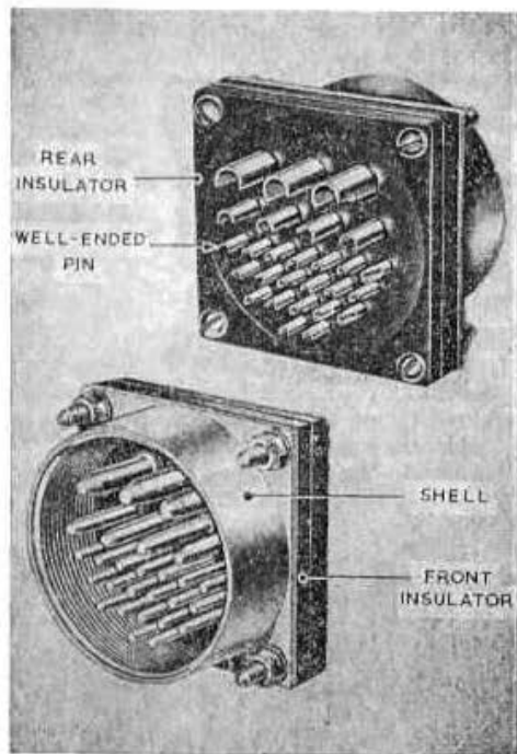
Fig. 2. Fixed unit—loose pins version
