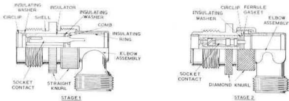
Fig. 14. Free unit (short reach), stages of development
