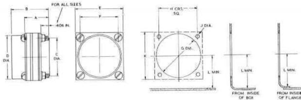
Fig. 22. Panel piercing details, fixed unit
