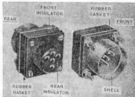
Fig. 3. Fixed unit—climatic-proof
