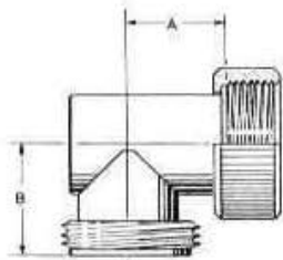
Fig. 40. Elbow assembly
