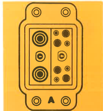
Example A shows an L 1390 and L 1387 side-by-side in a double-way shroud.
