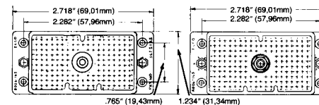
MALE RECEPTACLE (Exposed Contacts)
