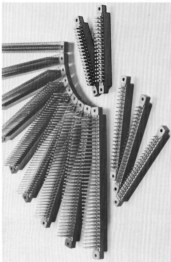
High Dielectric Strength Molding. HSD is glass-filled phenolic per MIL-M-14, type MFH. HMD is glass-filled diallyl phthalate per MIL-M-14, type SDG-F.
