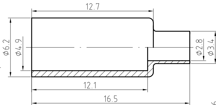
Crimp Ferrules
