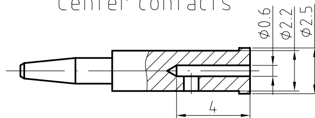
Center contacts
