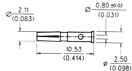
CENTER CONTACT
