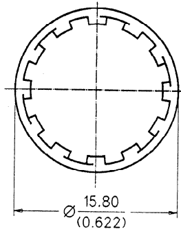
WASHER
