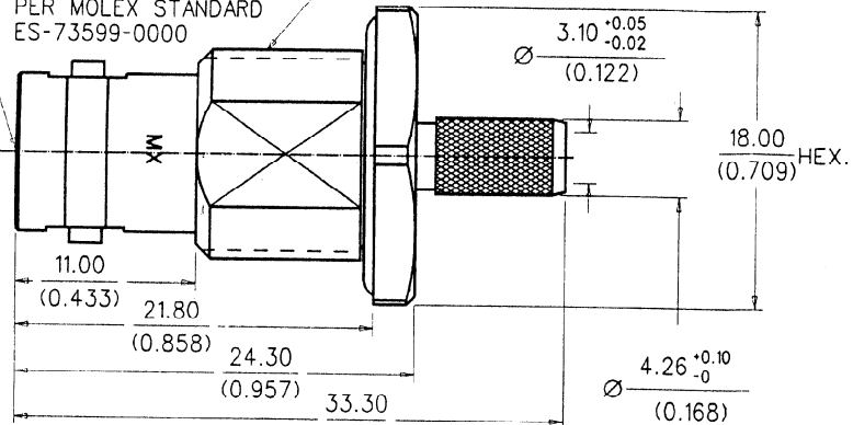
BODY ASSEMBLY
