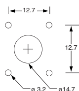
Panel Fixing Dimensions
