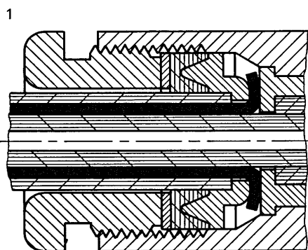
Cable-entry construction
