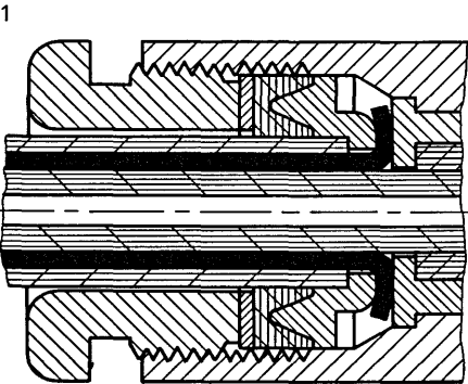
Cable-entry construction
