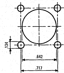
rear pane mounting
