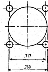
front panel mounting
