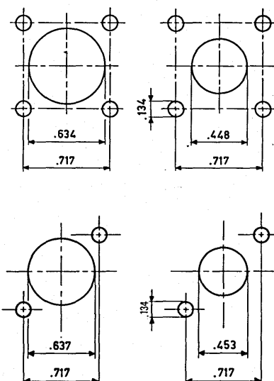
rear panel mounting
