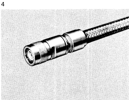
11C-50-7-3 with GK 103 fitted to cable RG-215/U
