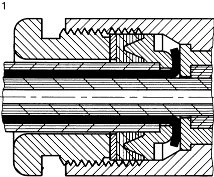
Cable-entry construction
