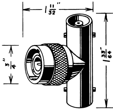
ADAPTER, TEE
