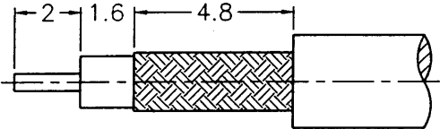
RECOMMENDED CABLE STRIPPING DIM'S (建議剝線尺寸)
