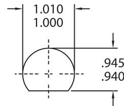
MOUNTING HOLE AE
