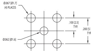
MOUNTING HOLE B
