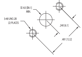
MOUNTING HOLE D
