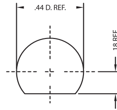
MOUNTING HOLE W
