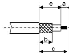
STRIPPING DIMENSIONS
