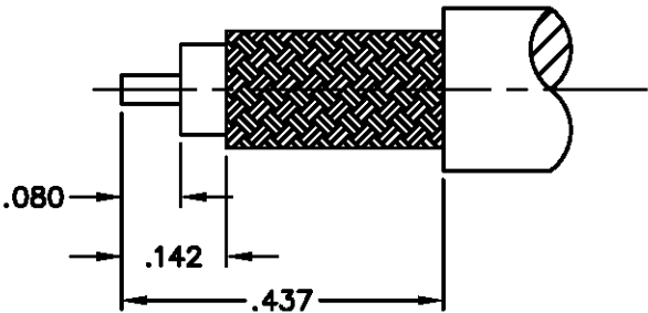
RECOMMENDED CABLE STRIPPING
