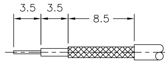
STRIP LENGTHS
