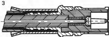
Crimp Version
