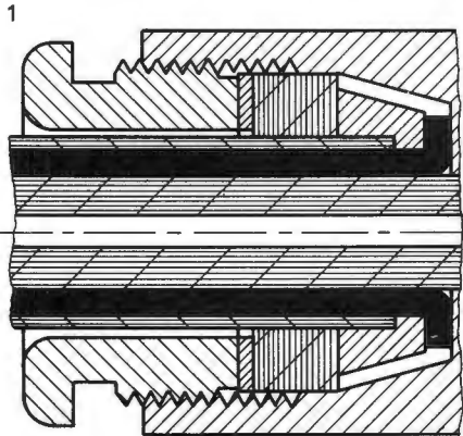
Cable-Entry Construction type 1
